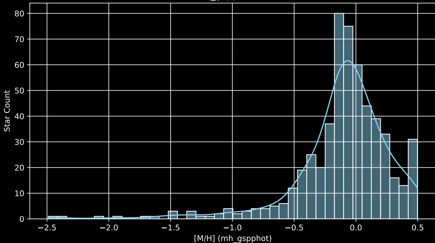
APOGEE DR17 Field: [PAL1 [M/H] (mh_gspphot) (n= 548)
