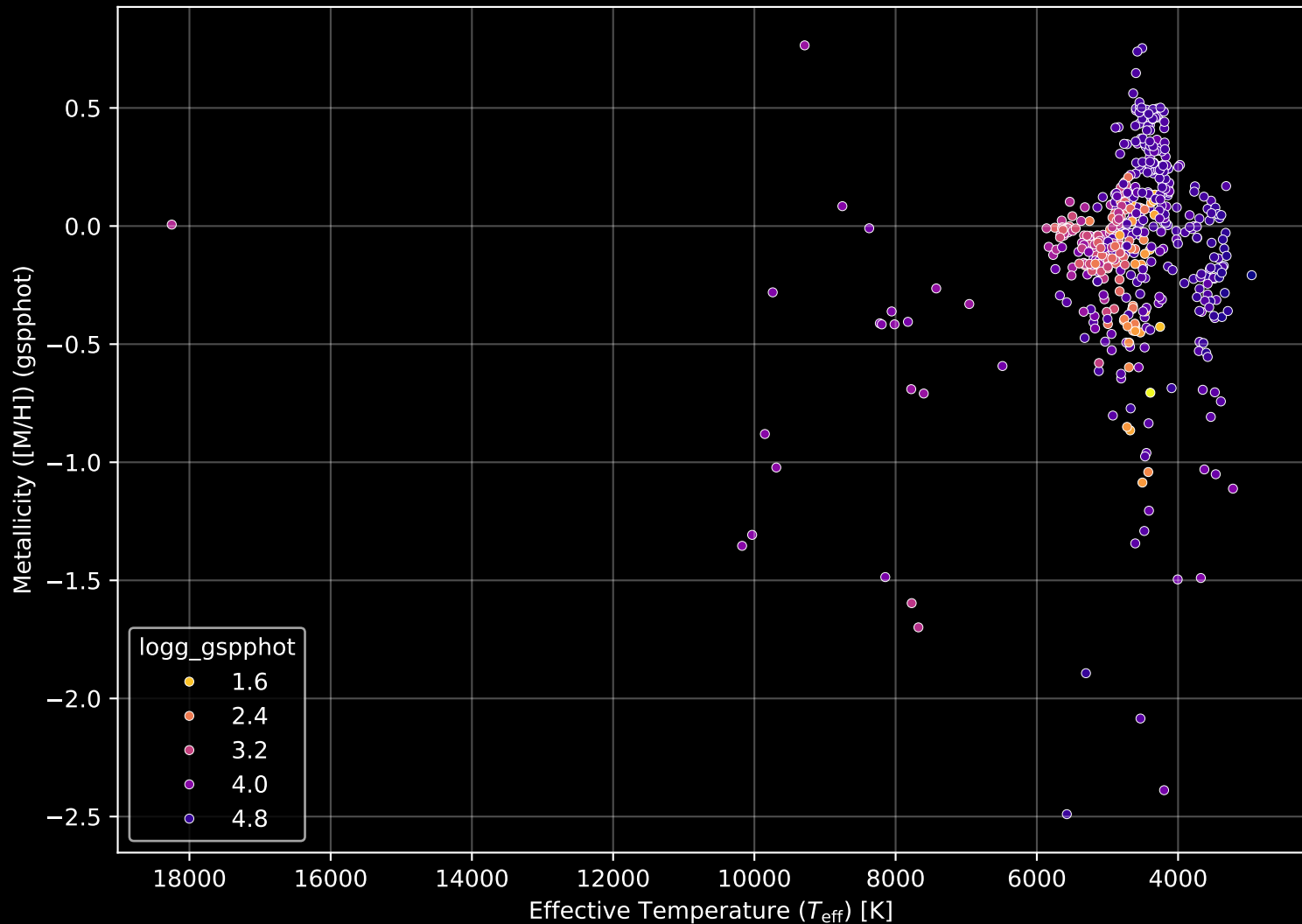
APOGEE DR17 Field: [PAL1] Stellar Population Parameters (n= 558)
