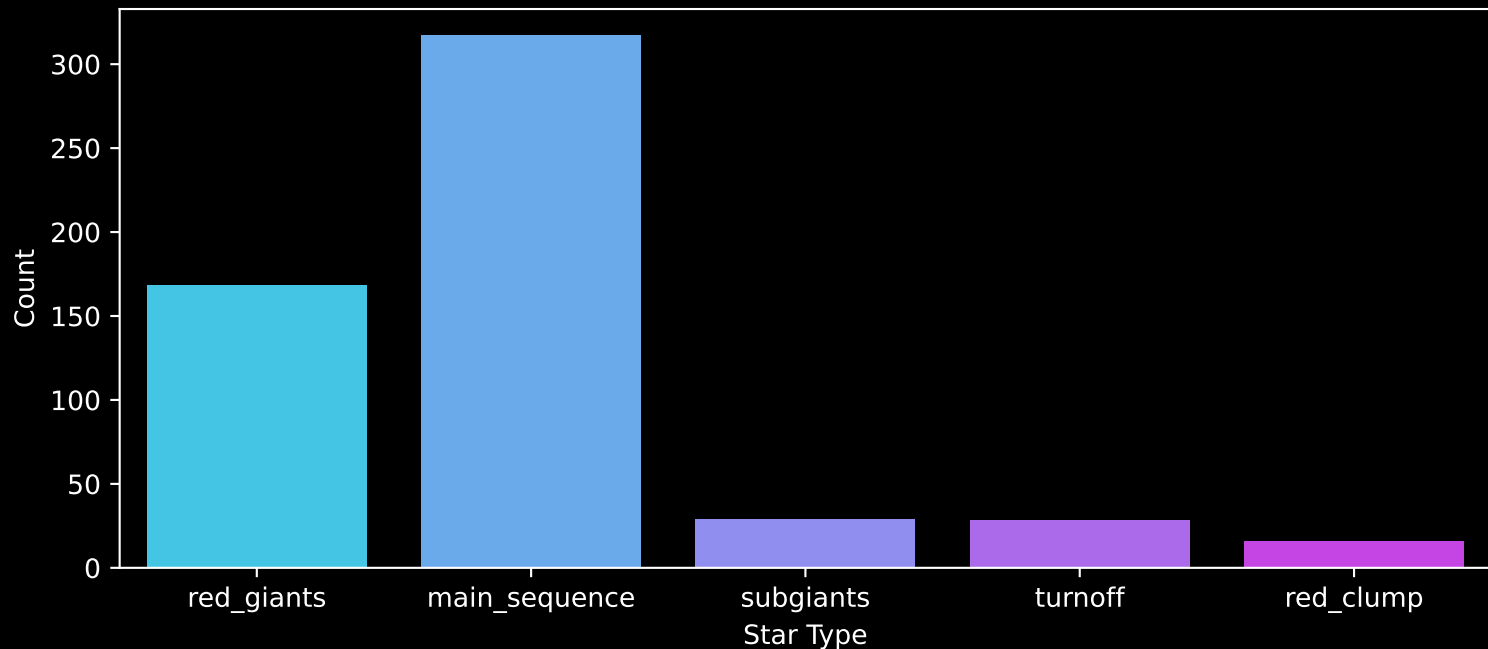
APOGEE DR17 Field: [PAL1] Count plot of Star Type
