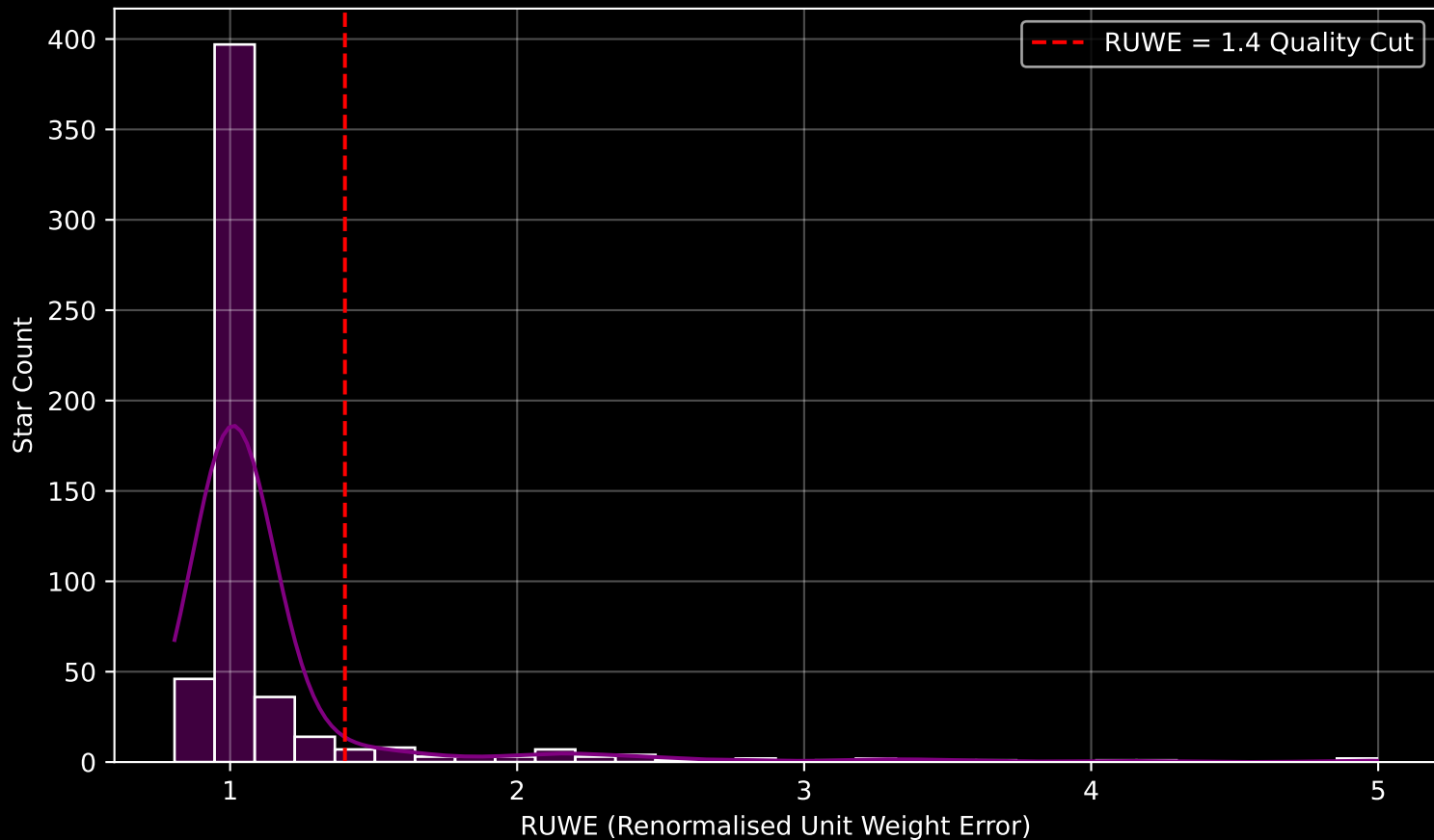
GAPOGEE DR17 Field [PAL1] RUWE Distribution (n= 545)
