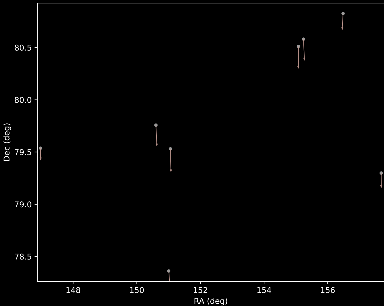
APOGEE DR17 Cluster 11 Proper Motion Vectors (n=8)
