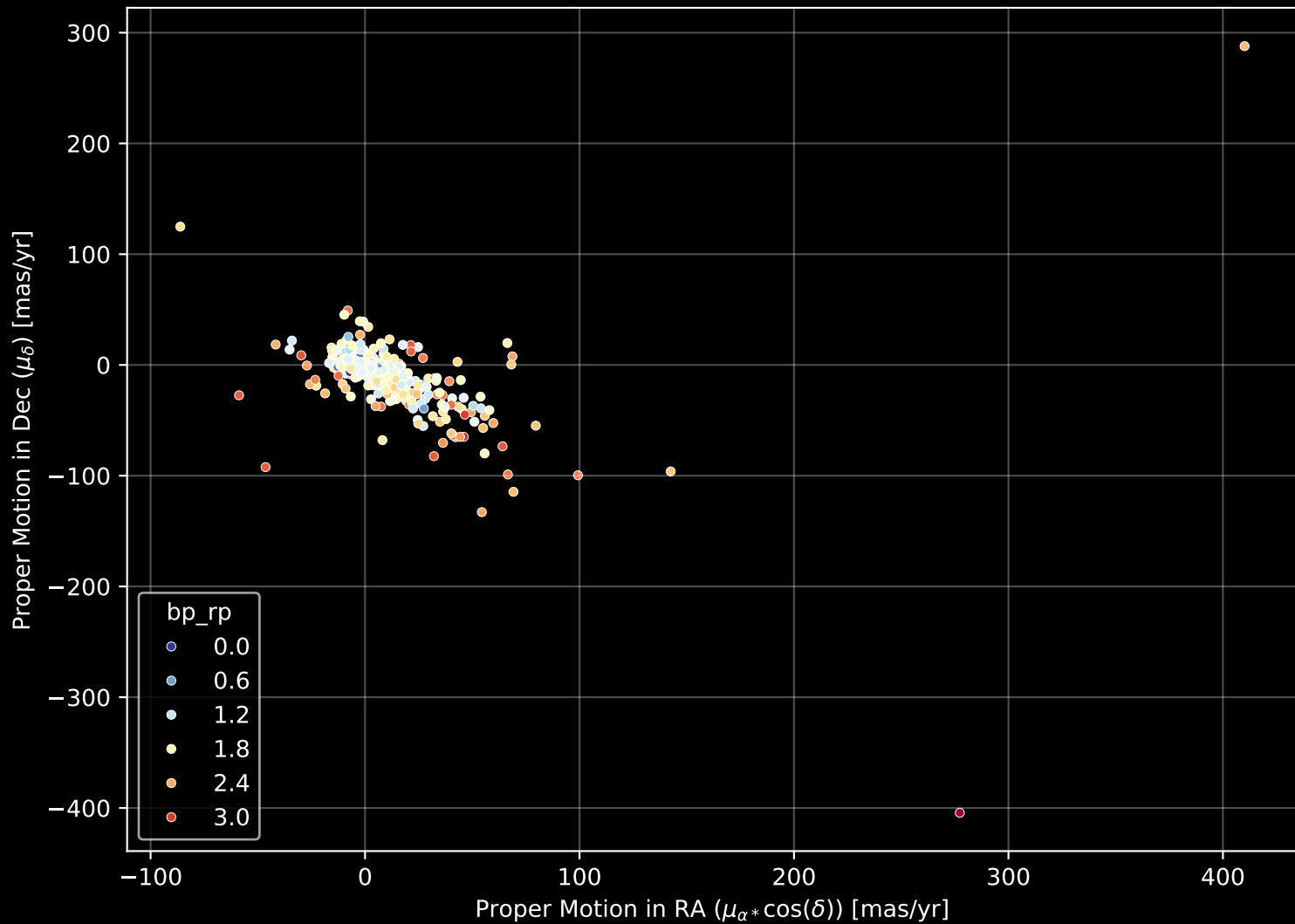
APOGEE DR17 Field: [PAL1] Proper Motion Diagram (n= 558)
