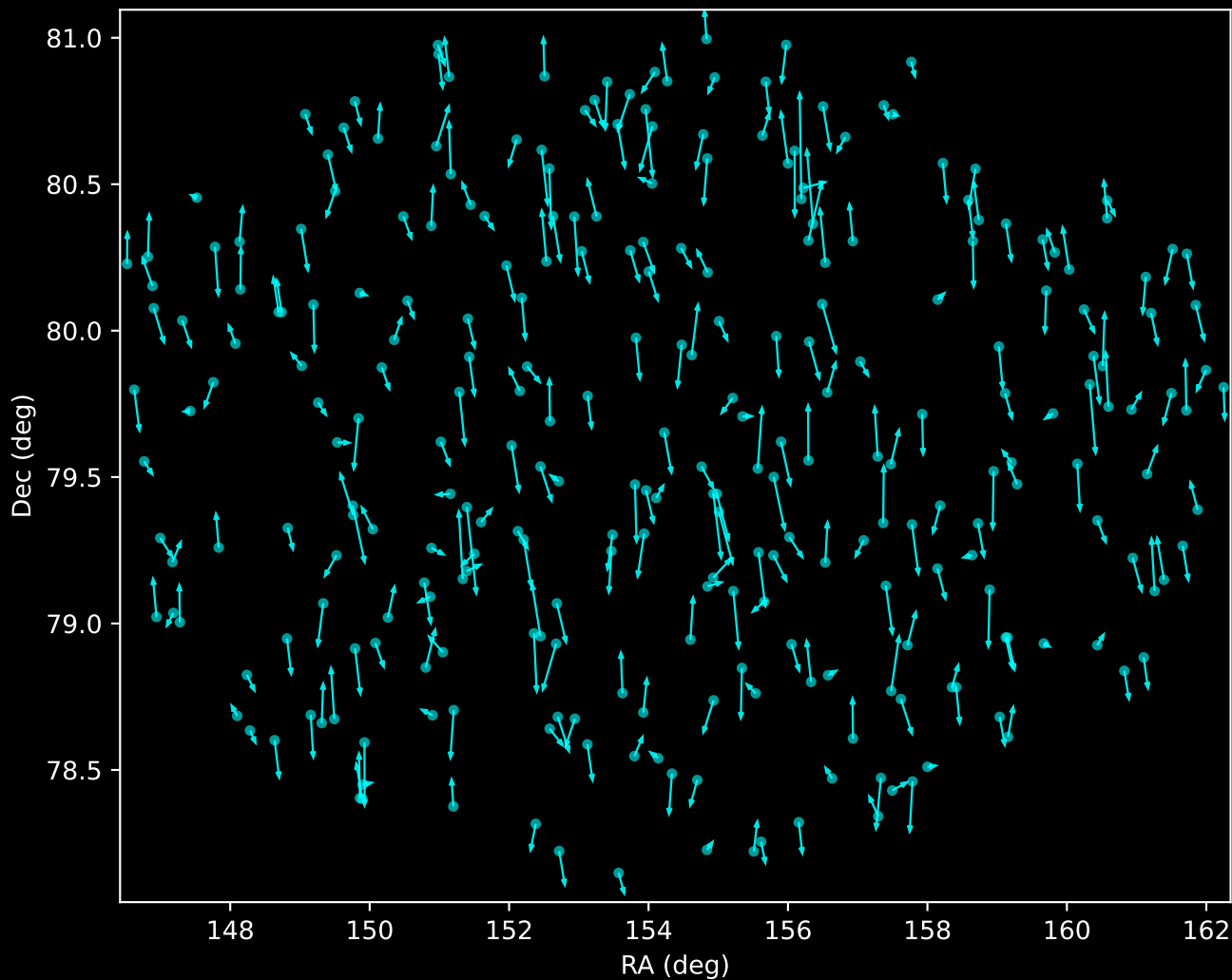
APOGEE DR17 Noise Stream Proper Motion Vectors (n=277)
