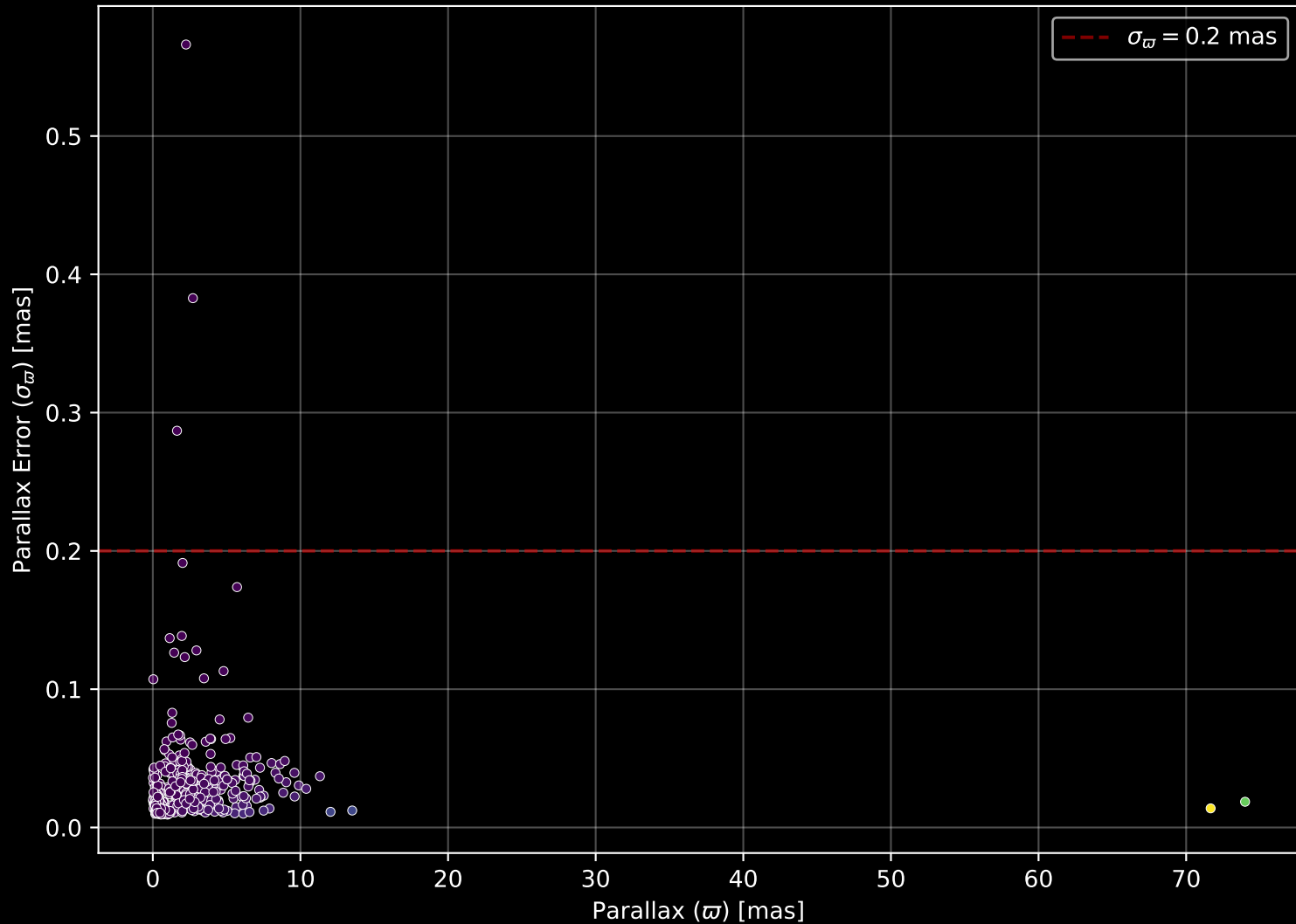
APOGEE DR17 Field: [PAL1] Parallax Quality (n= 558)
