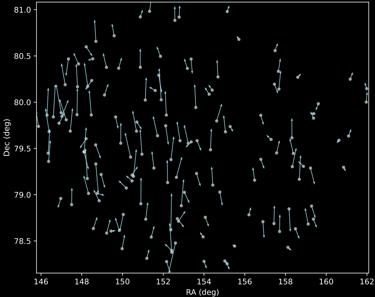
APOGEE DR17 Cluster 19 Proper Motion Vectors (n=144)
